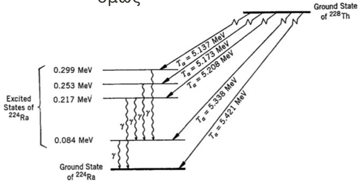
Fig. 4.1 α-particle transitions observed in the decay of ^{228}\text{Th} .
