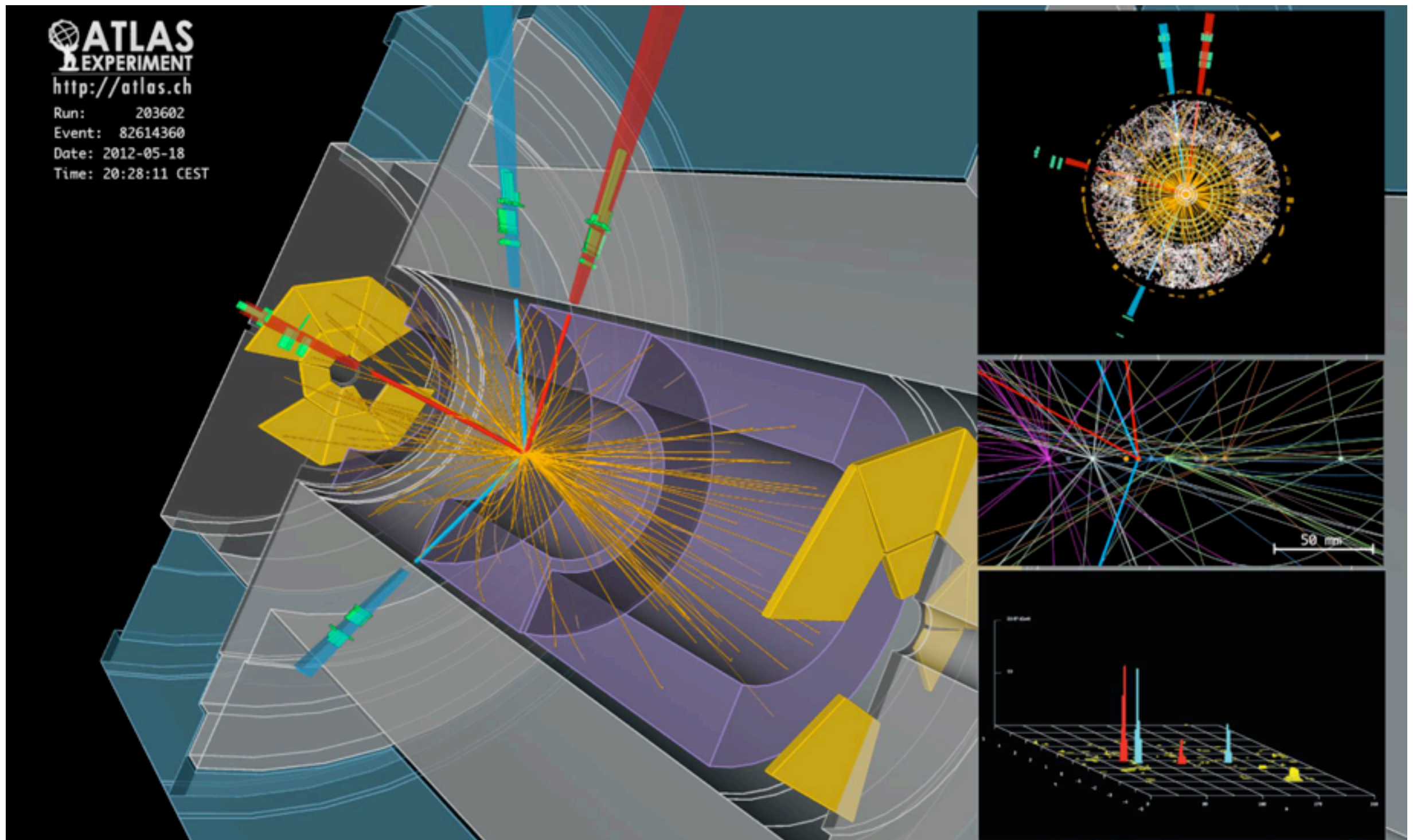
A Higgs candidate decaying to 4e: Mass= 124.6 GeV
