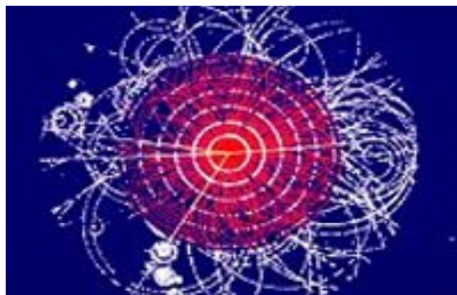
Particle Physics
