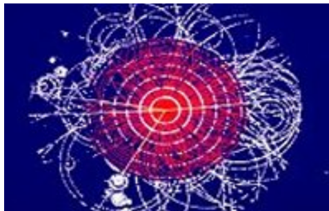
Particle Physics
