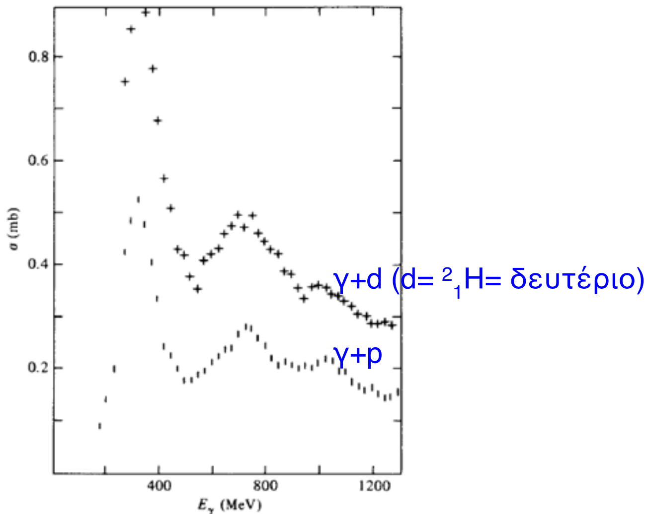
Fig. 3.1 The total photon cross-section for hadron production on protons (dashes) and deuterons (crosses). The difference between these cross-sections is approximately the cross-section on neutrons. (After Armstrong, T. A. et al. (1972), Phys. Rev. D5 , 1640; Nucl. Phys. B41 , 445.)
